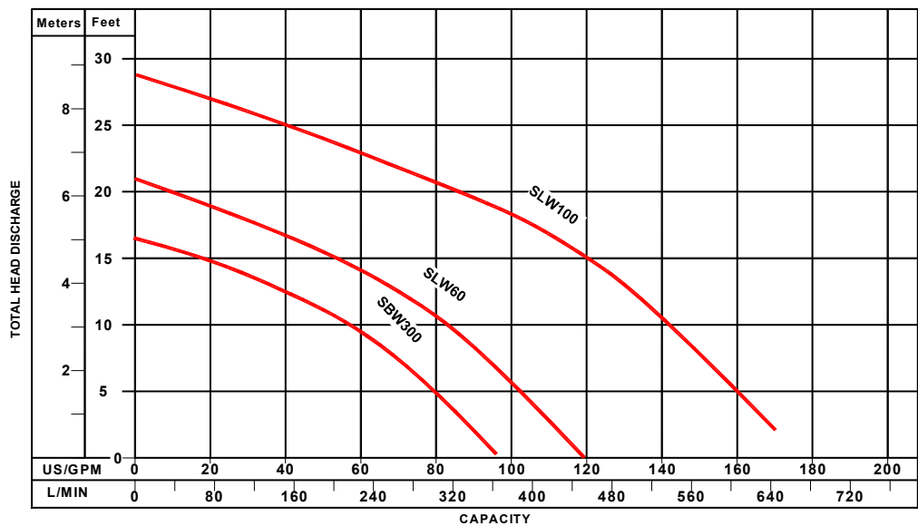
PUMPING CURVES SBW / SLW SERIES
