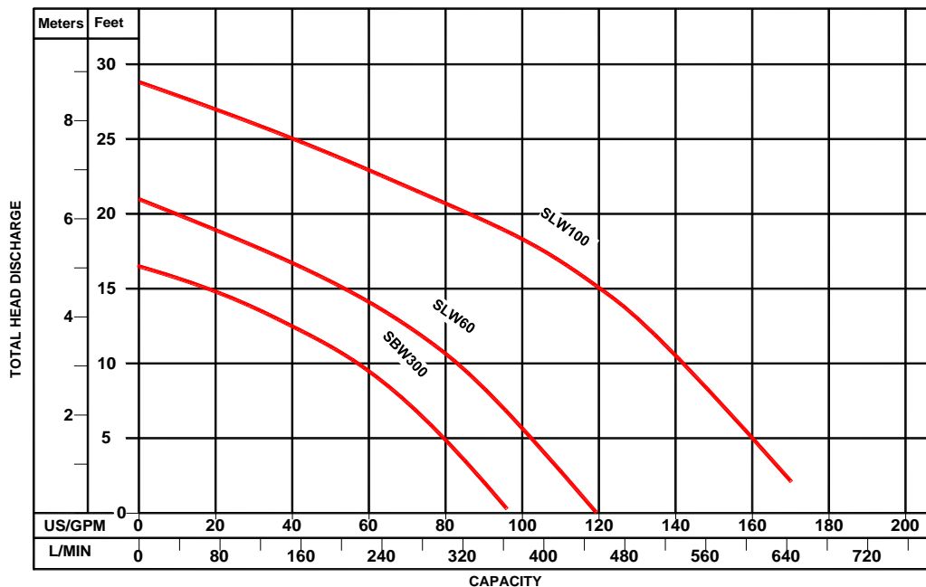
PUMPING CURVES SBW / SLW SERIES
